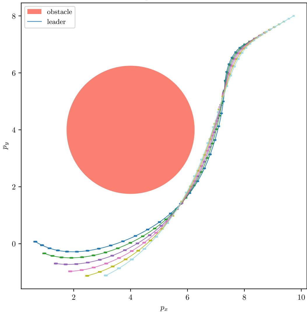
6-vehicle platoon reach tube
