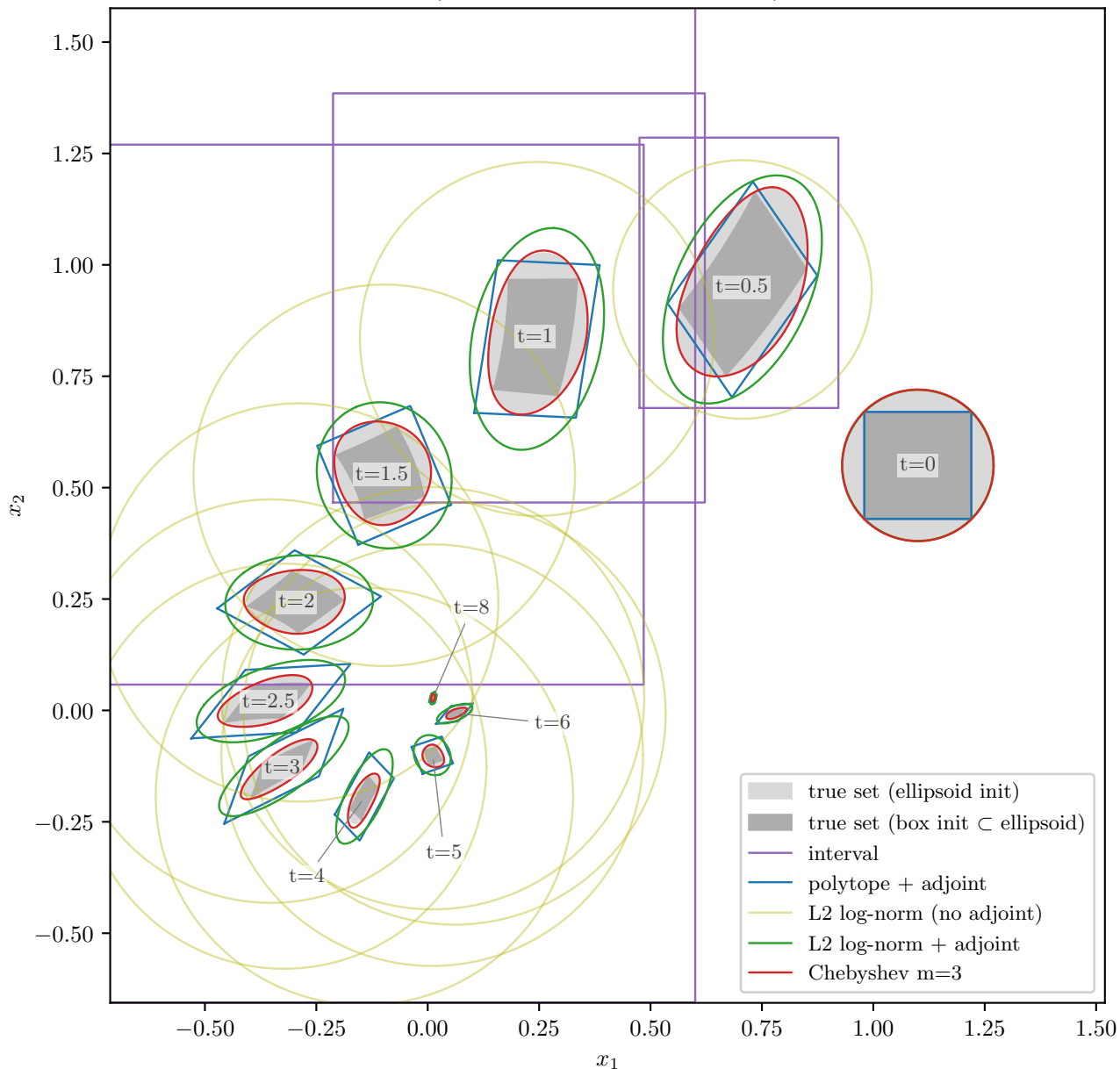
Reverse Van der Pol, box (1.10, 0.55) \pm 0.12 and its circumscribed ellipsoid ( dt=0.005 , snapshots to t=8 )
