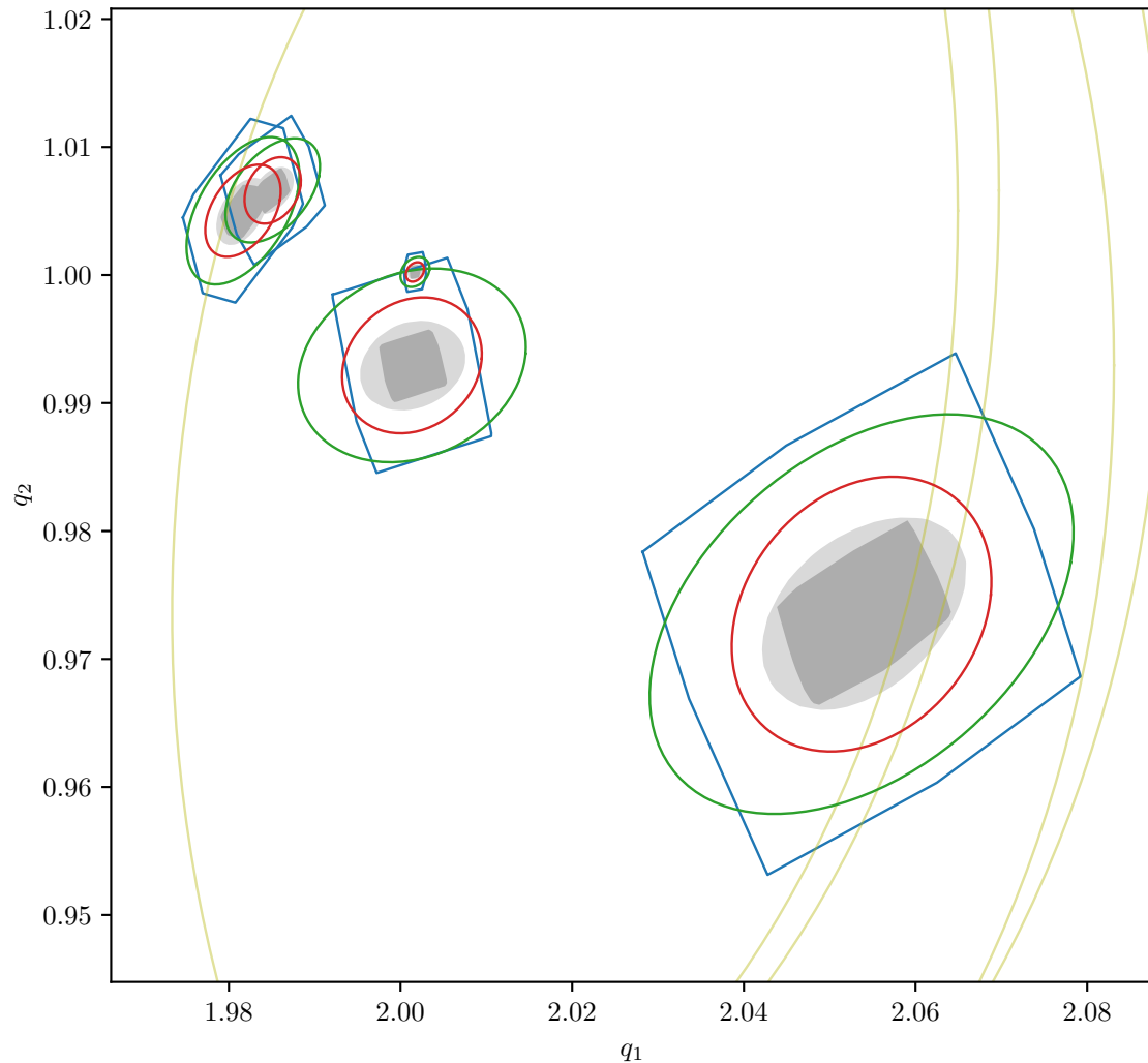
zoom at the setpoint ( t \geq 5 )
