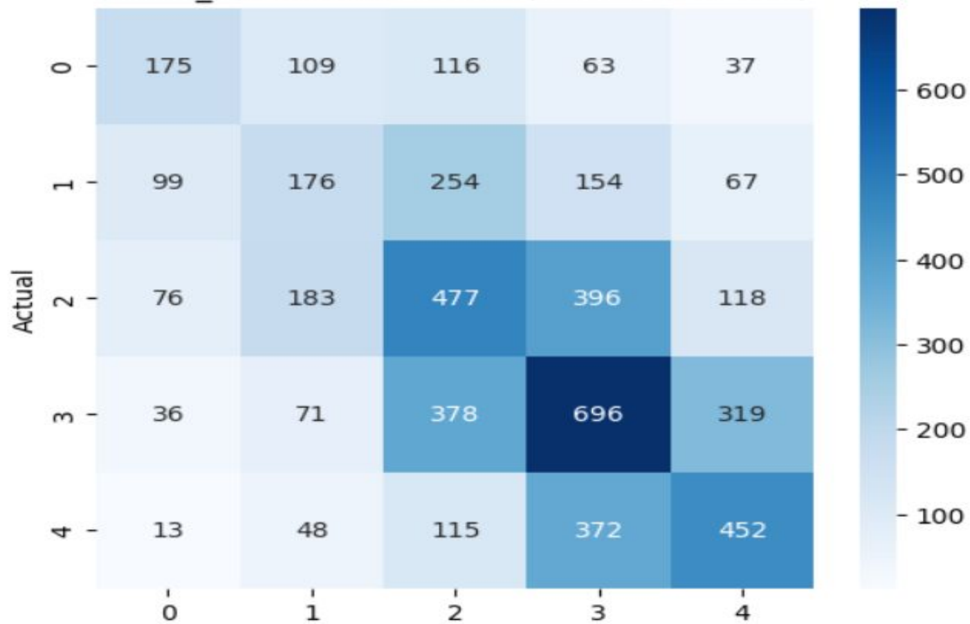
Model_B Confusion Matrix (Imbalanced Test)
