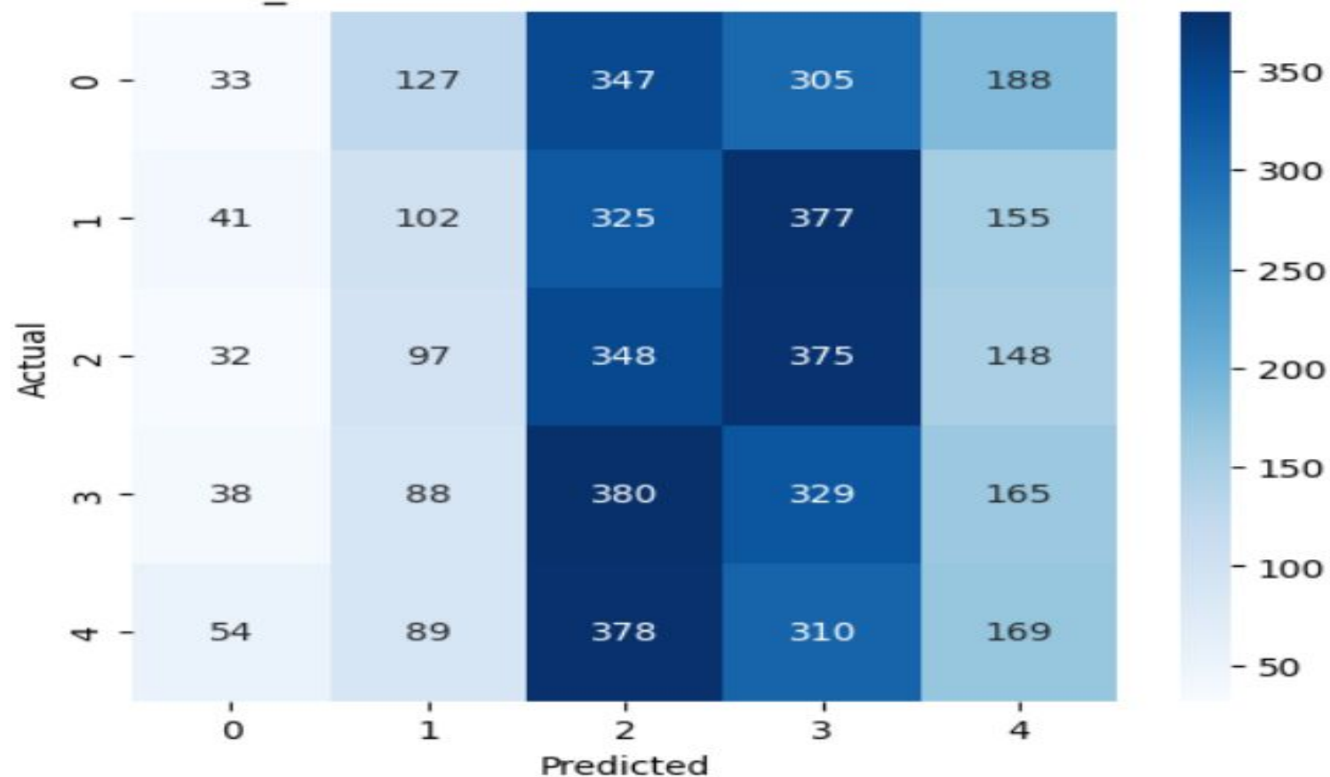
Model_B on Balanced Test - Confusion Matrix
