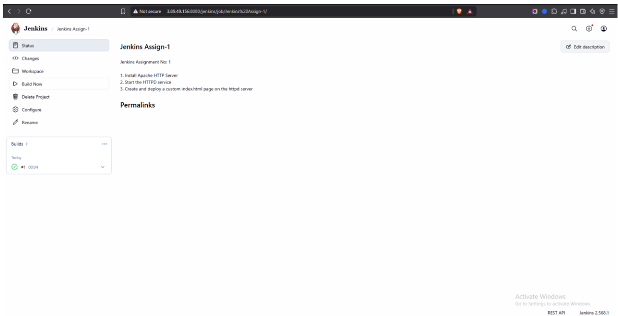
Figure 2: Jenkins Job
