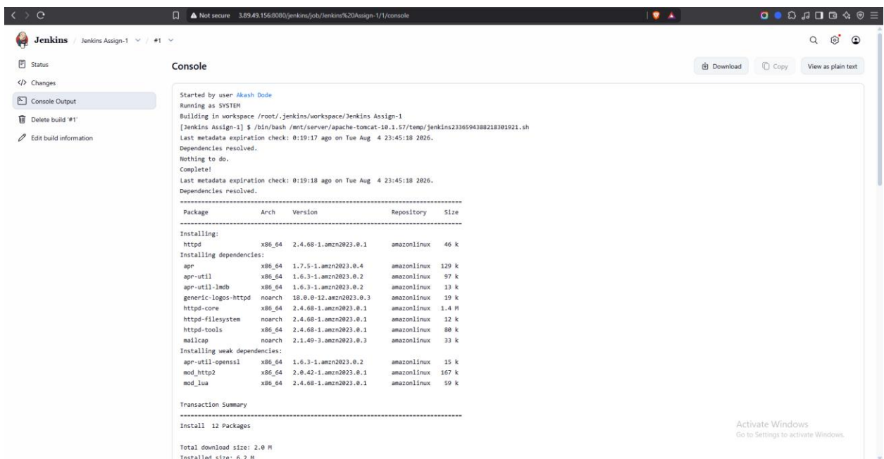
Figure 3: Console Output
