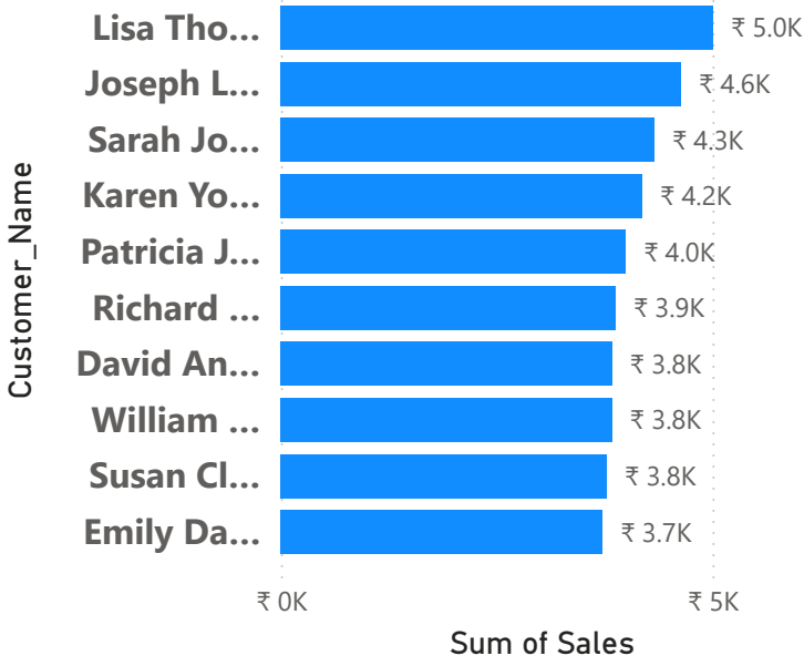
Top 10 Customers
