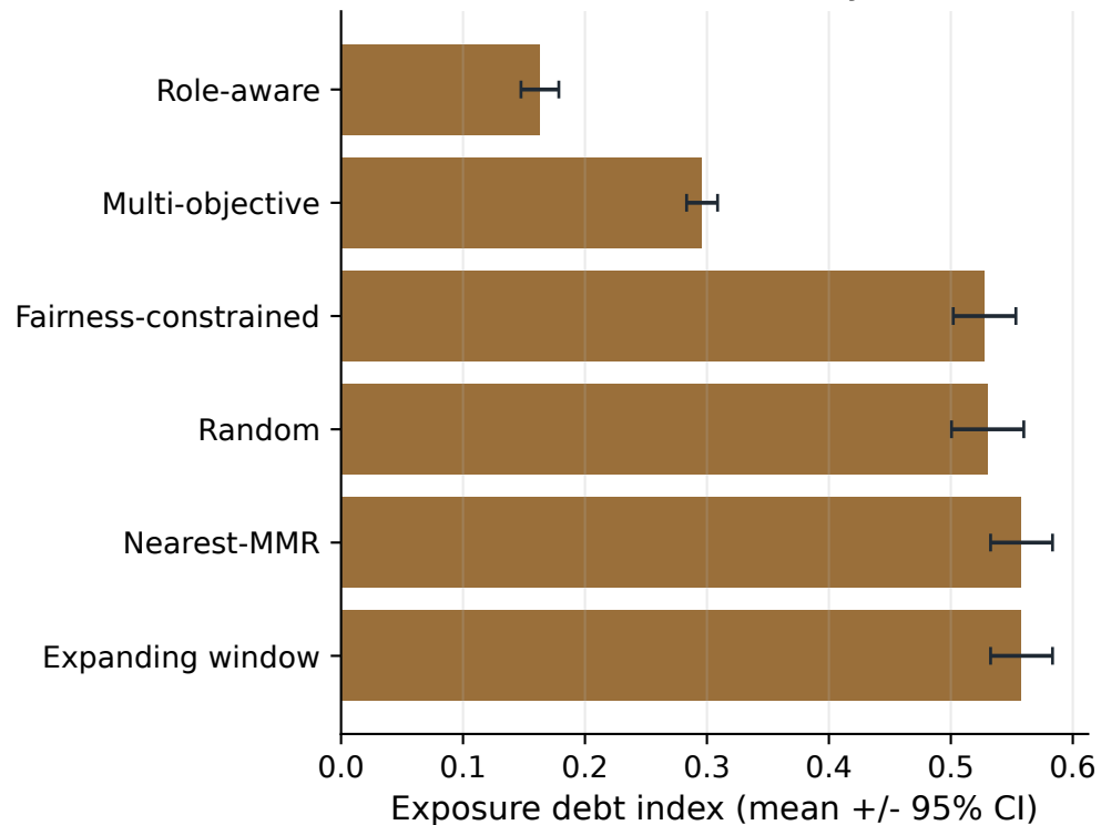
Team-formation layer
