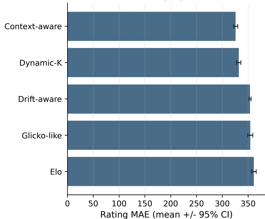
Rating layer
