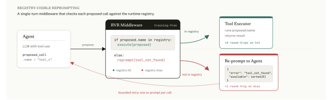
Figure 3. RVR middleware. An O(1) membership check runs in-process on each proposed call. Hits execute. Misses trigger one re-prompt with a structured tool_not_found envelope (and the sorted registry under C_1 ). The no-violation path adds zero provider round-trips; the violation path adds one, bounded to a single retry.
