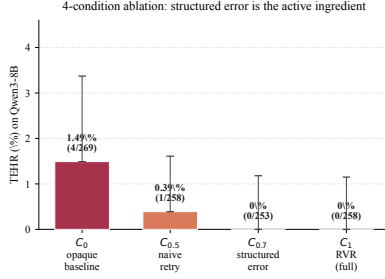
Figure 1. Qwen3-8B 4-condition ablation. The structured-error envelope (C 0.7 ) drives the prevention; adding the registry list (C 1 ) adds no further reduction.
