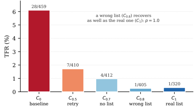
Figure 7. Qwen2.5 ablation ladder. A bare retry ( C_{0.5} ) only halves the 6.10% baseline, while the structured tool_not_found envelope cuts it about 20 \times ; a wrong registry list ( C_{0.8} ) recovers as well as the real one ( C_1 ; Fisher p = 1.0 ), so recovery is format-driven.
