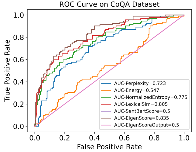
Fig. 1. ROC curves on CoQA, without feature clipping. The entries “SentBertScore” and “EigenScoreOutput” are placeholders at 0.5 because the sentence-similarity model was not used.
