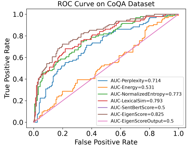
Fig. 2. ROC curves on CoQA, with feature clipping.
