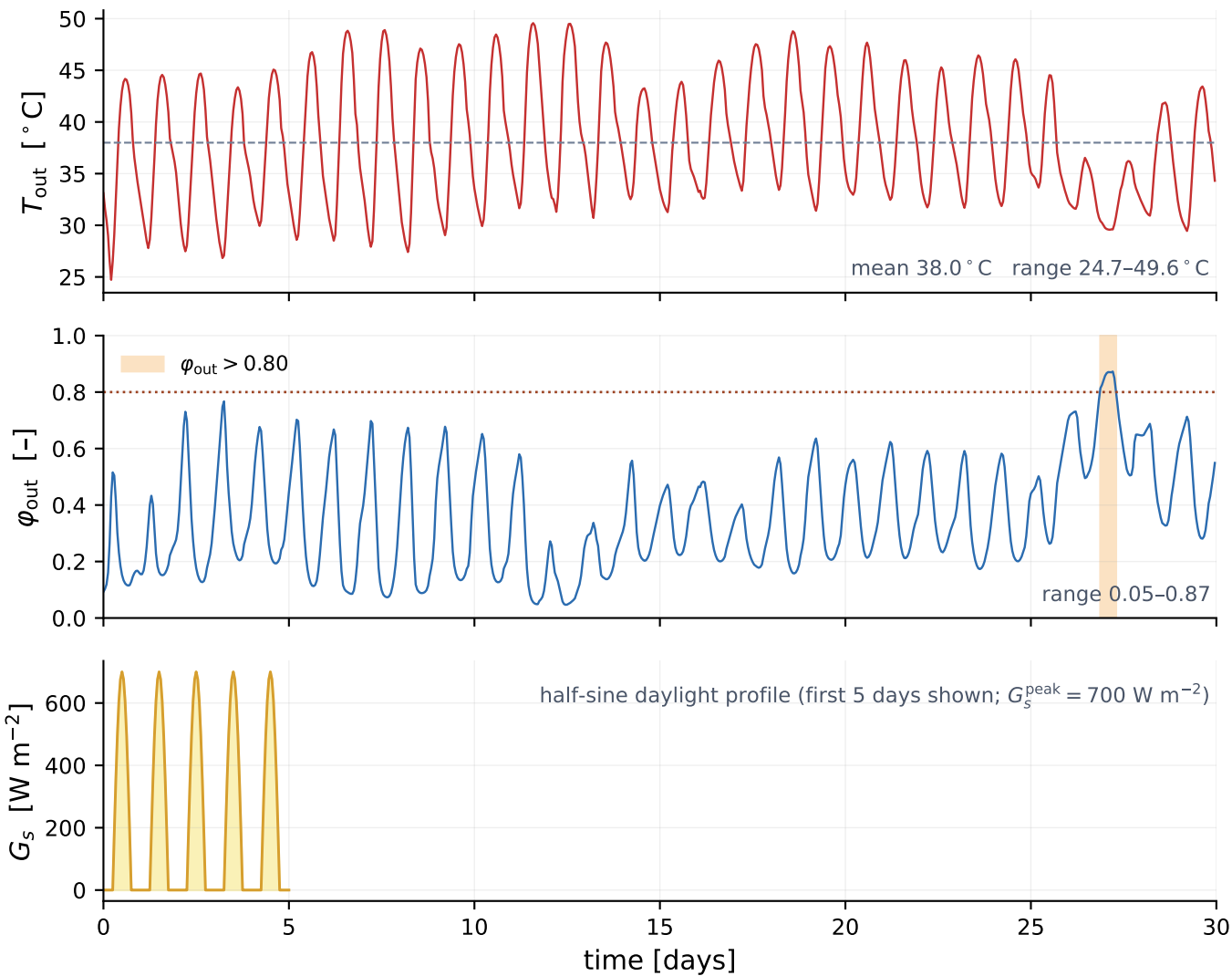
NASA POWER MERRA-2 reanalysis forcing, Sukkur (27.70° N, 68.86° E), 1–30 June 2025
