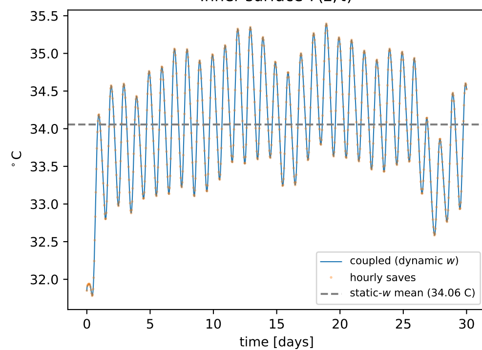
Inner surface T(L, t)
