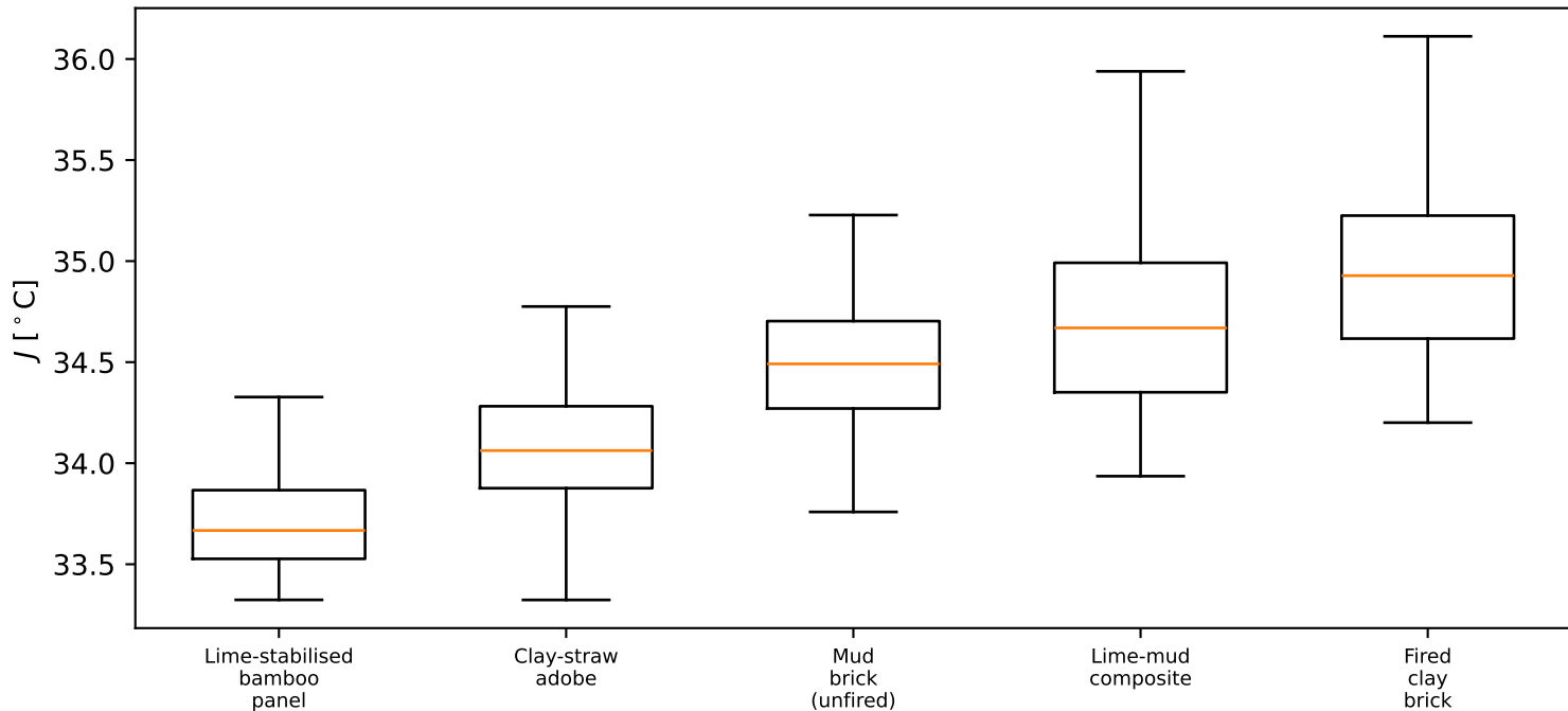
Inner-surface temperature under correlated property uncertainty (64 FDM replicates)
