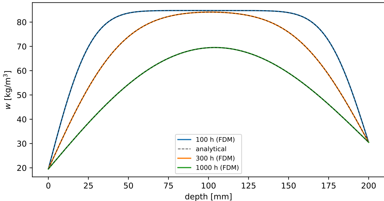
HAMSTAD Benchmark 2: isothermal drying of a 200 mm layer
