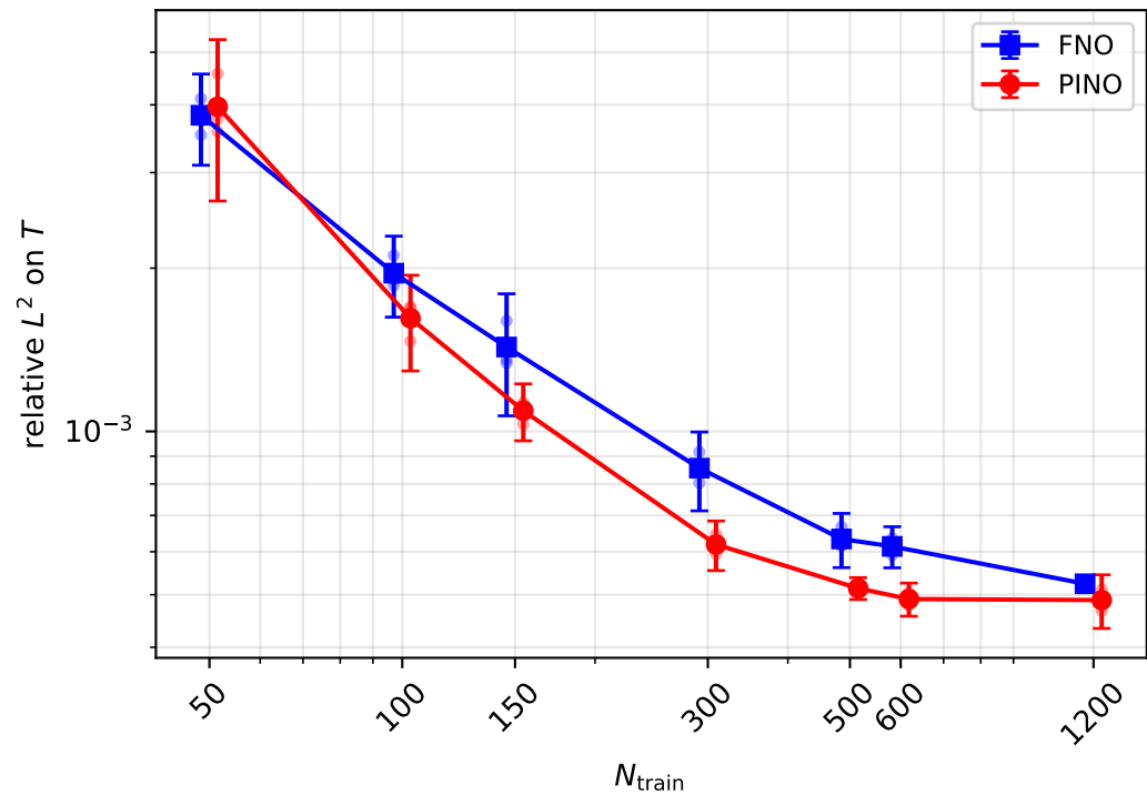
Data efficiency: mean \pm 95% CI over seeds (dots: individual runs)
