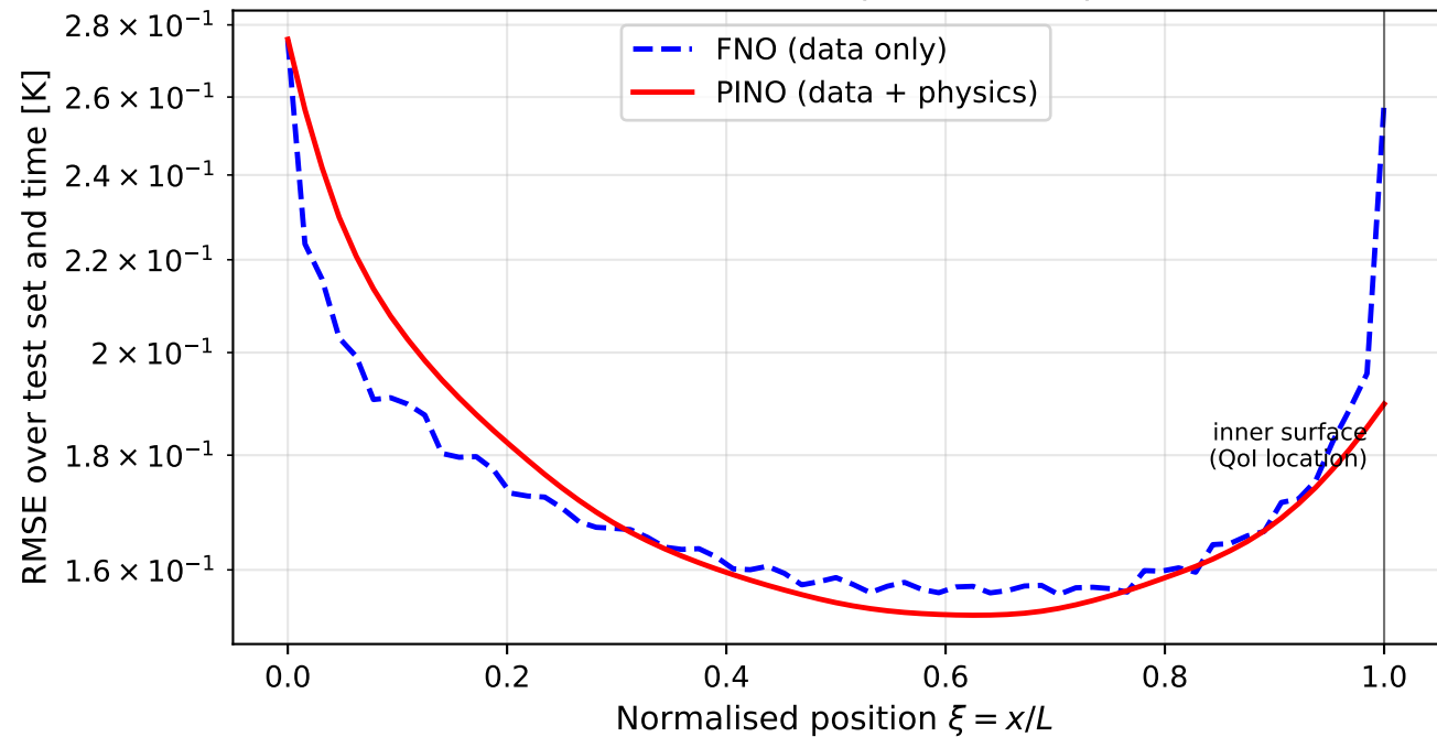
Where the PDE loss helps: error vs. position
