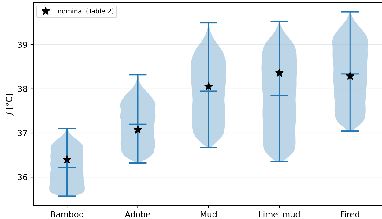
(a) Peak inner-surface temperature under property uncertainty
