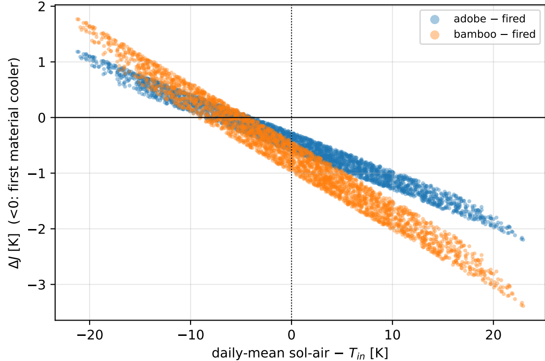
(b) sign of \Delta J is set by mean sol-air vs T_{in}
