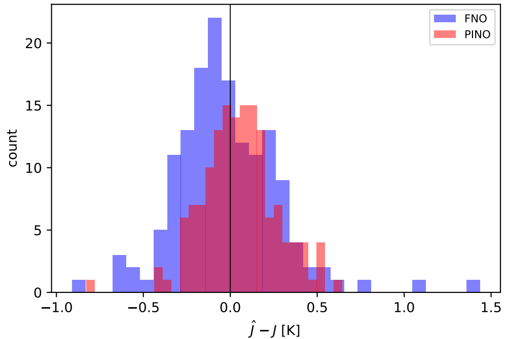
(b) PINO: MAE=0.167 K, R^2=0.9976
