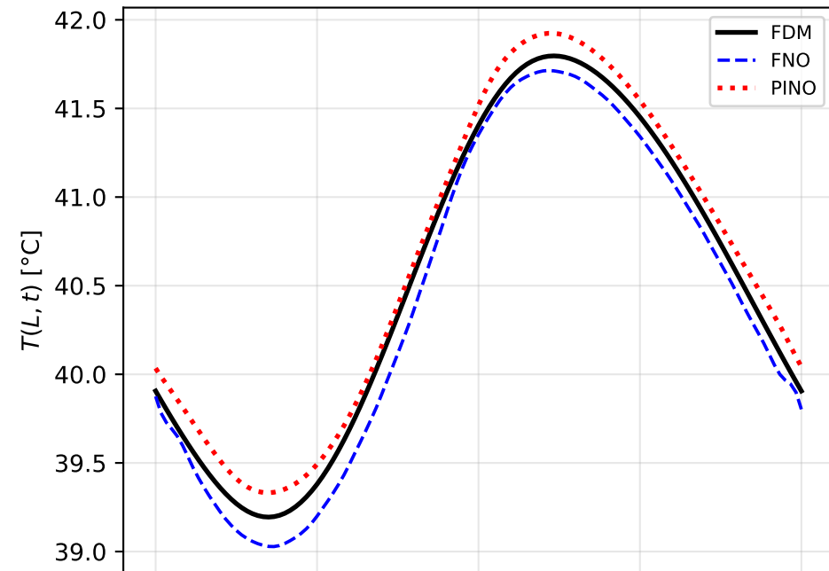
median PINO |\Delta| = 0.128 K (test idx 13)
