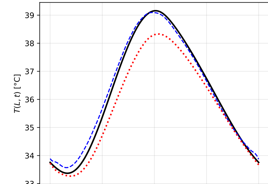
worst PINO |\Delta| = 0.830 K (test idx 45)
