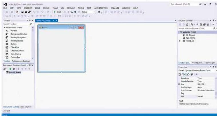
Gambar 5.2 Form1
