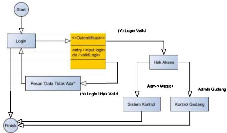
Gambar 2.3 Statechart Diagram
