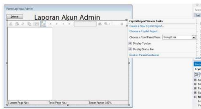
Gambar 8.19 Form LapViewAdmin
