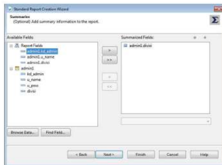
Gambar 8.14 Jendela Summaries
