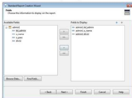
Gambar 8.12 Seleksi Field
