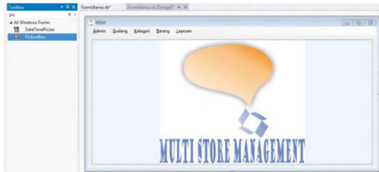
Gambar 6.6 FormUtama
