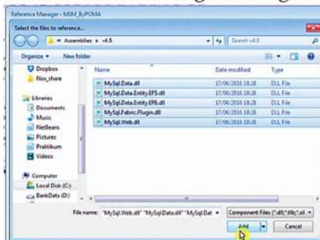
Gambar 5.5 Connector Net
