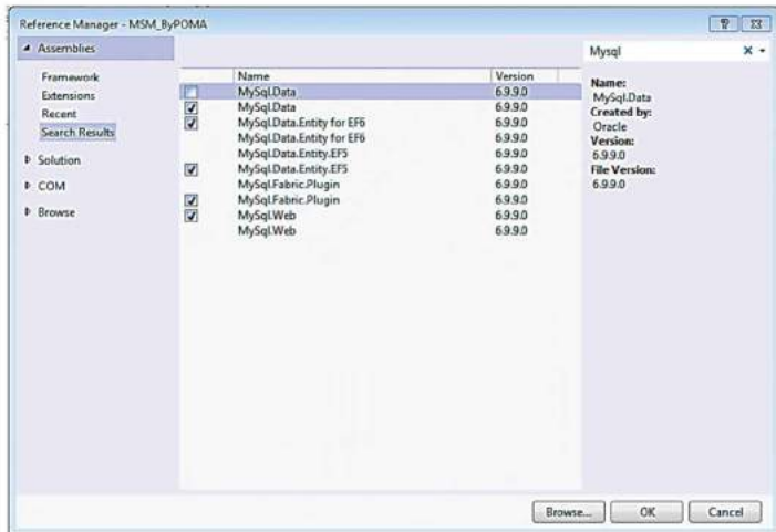
Gambar 5.6 Reference Manager
