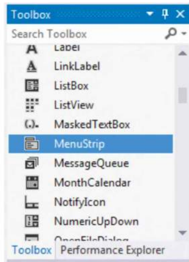
Gambar 6.4 ToolBox
