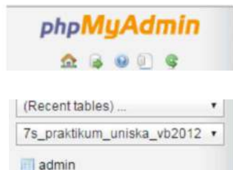
Gambar 3.5 Tabel admin
