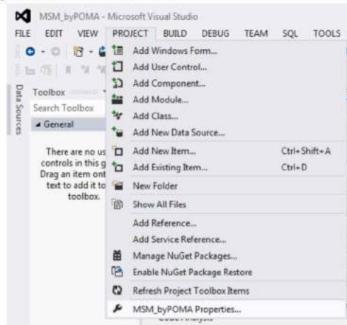
Gambar 7.2 Project Properties
