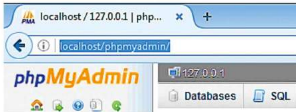
Gambar 3.1 localhost
