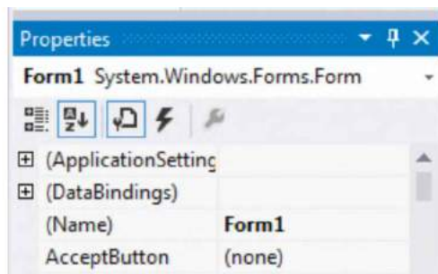
Gambar 6.1 Jendela Properties
