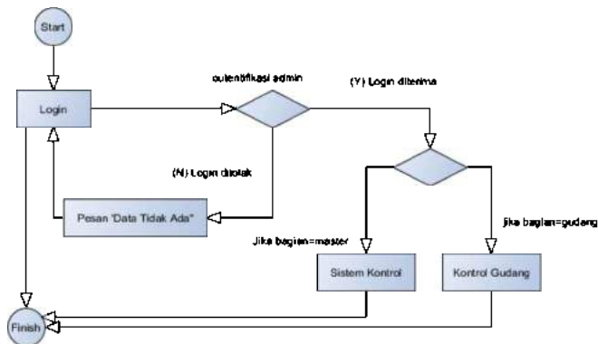
Gambar 2.4 Activity diagram
