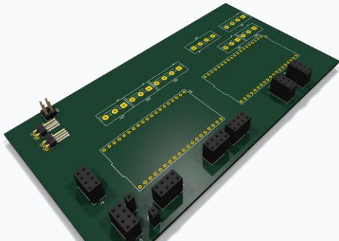
Gambar 3.2: Render 3D Custom Controller PCB KiCad
