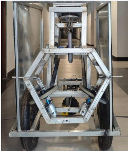
Gambar 3.1: Fisik Robot Pelatih Kiper (Swerve Drive & Tri-Spinner)
