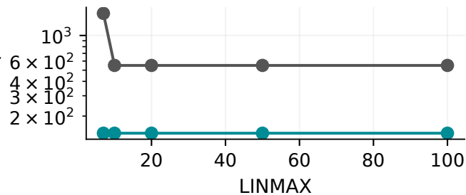
Residual evaluations
