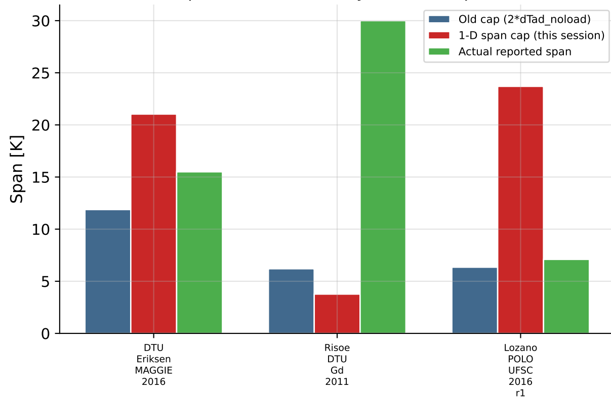
Span Reach: Old Cap vs. 1-D Model vs. Reality (bar at "actual span" not reached by the 1-D cap = still infeasible)
