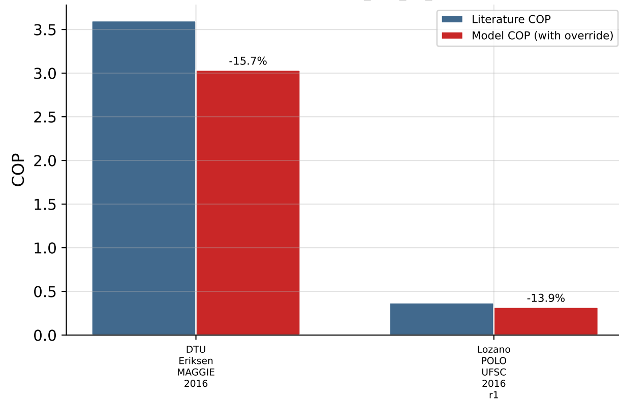
COP Recovered by the Override (% label = model error vs. literature) Still infeasible: Risoe_DTU_Gd_2011
