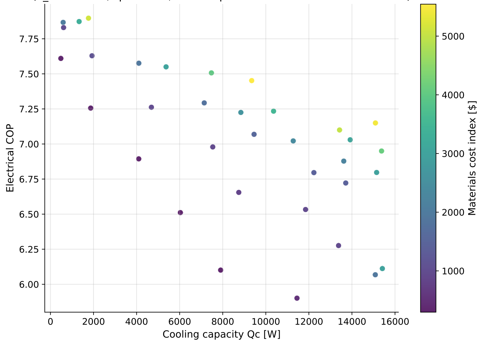
NSGA-III Pareto-Optimal AMR Designs ( T_{\text{cold}}=291\text{K} , span=10K; state-dependent loss + NTU thermal model)
