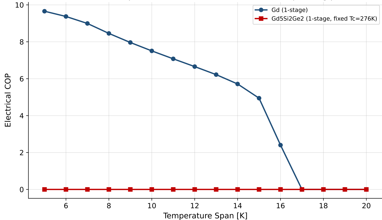
Gd vs. Gd 5 Si 2 Ge 2 in the ASHRAE Range (Gd 5 Si 2 Ge 2 collapses to ~0: its fixed T c is far from the operating point)
