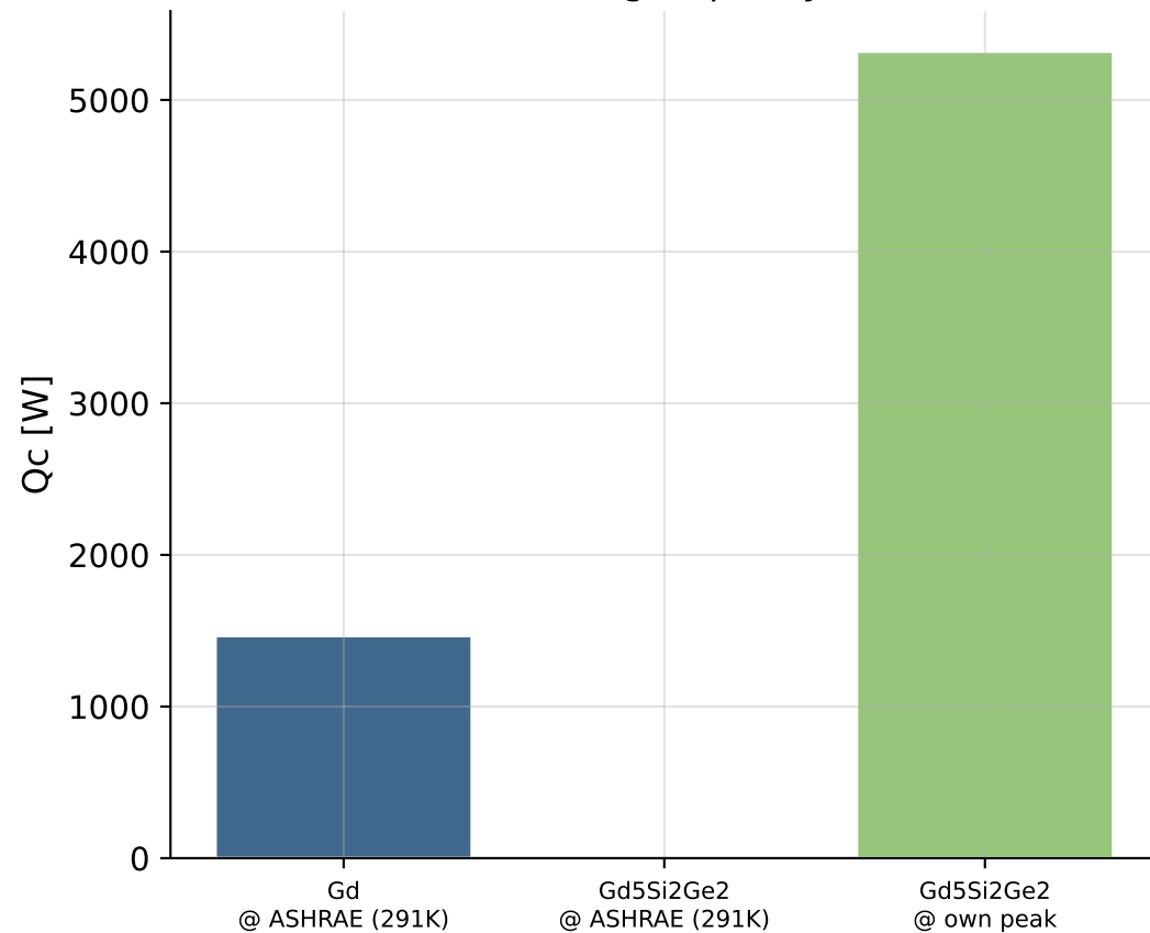
Cooling Capacity
