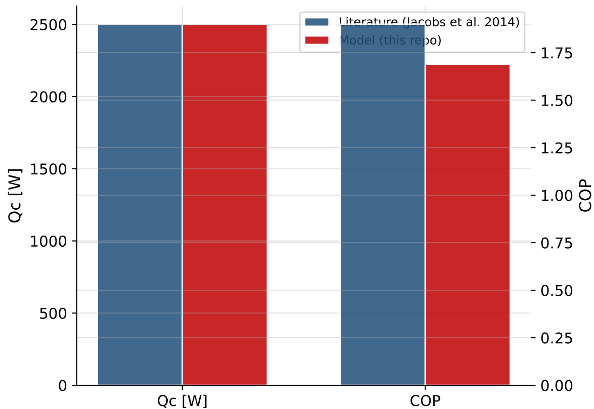
Astronautics_rotary_2014 Validation COP error: -11.1%
