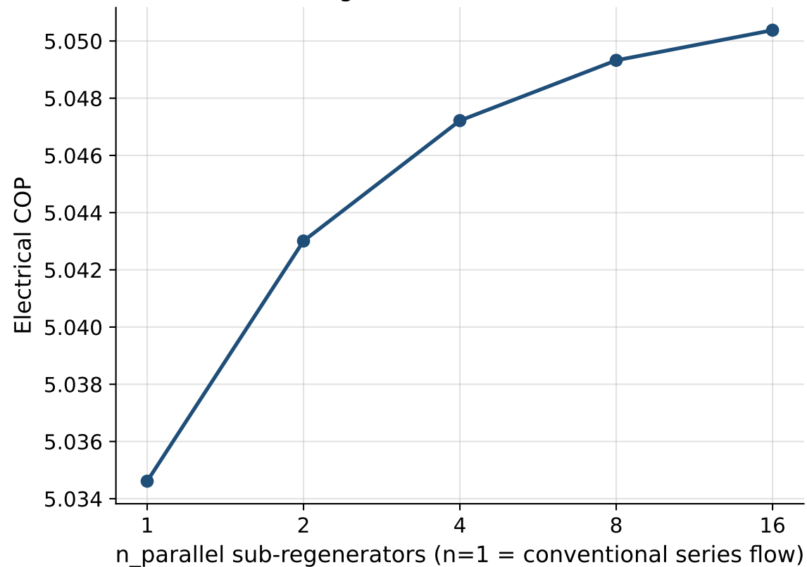
COP vs. Hypereg Split ( \dot{m}=0.08\text{kg/s} baseline — benefit saturates)
