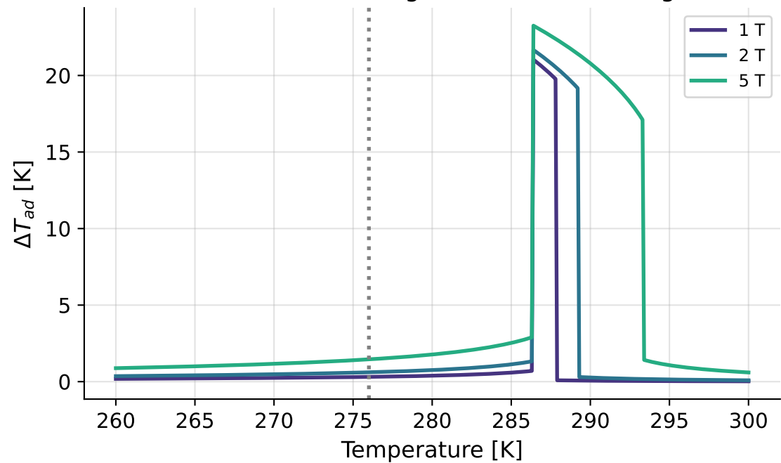
Adiabatic Temperature Change (uncorrected — see Giguère cross-check, Fig. 04)
