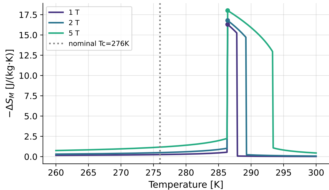
Isothermal Entropy Change (first-order Landau model)
