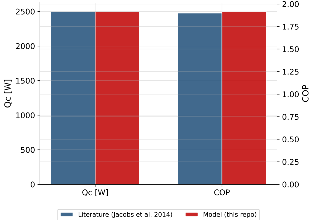
Astronautics_rotary_2014 Validation COP error: +1.0%
