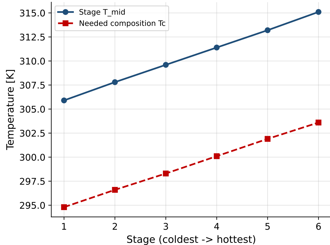
6-Layer Curie-Graded Bed: Stage Temperature vs. Needed Composition
