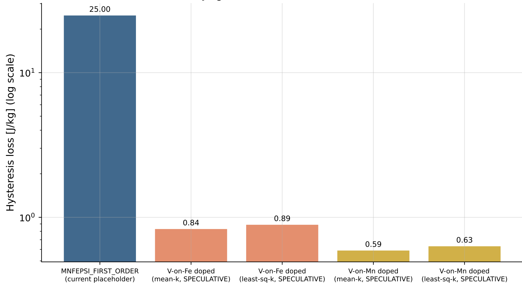
SPECULATIVE: V-Doped (Mn,Fe) 2 (P,Si) Hysteresis-Loss Estimate vs. Current 25.0 J/kg Placeholder (Phase 36, not a new default)
