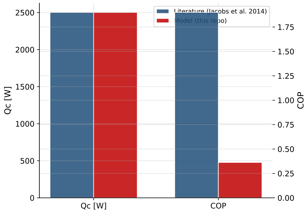
Astronautics_rotary_2014 Validation COP error: -80.9%
