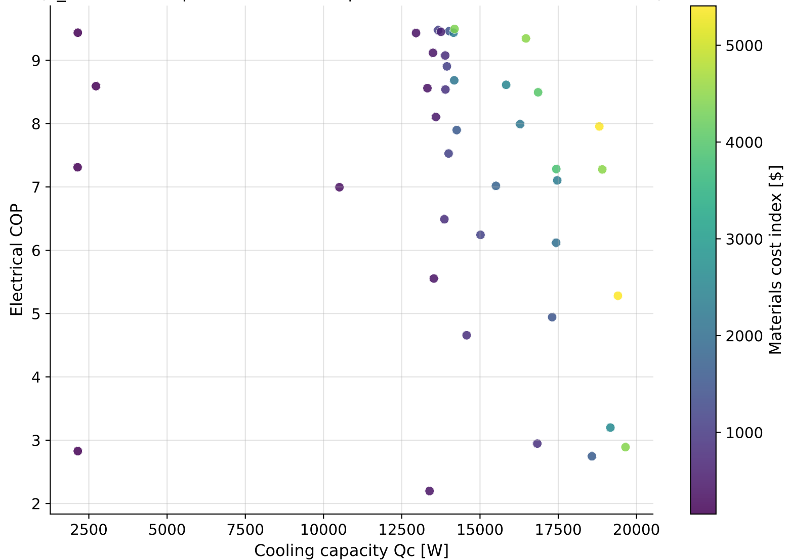
NSGA-III Pareto-Optimal AMR Designs ( T_{\text{cold}}=291\text{K} , \text{span}=10\text{K} ; state-dependent loss + NTU thermal model)
