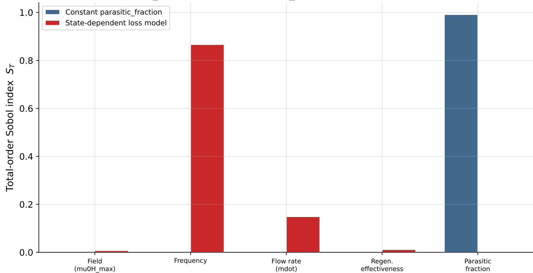
Sobol Sensitivity of Electrical COP ( T_{\text{cold}}=291\text{K} , span=10K, N_{\text{base}}=64 Saltelli samples)
