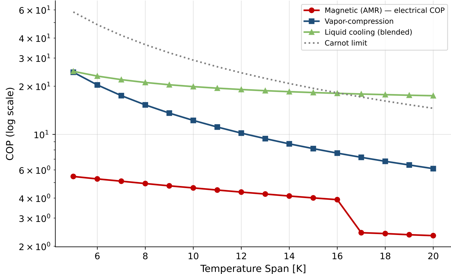
Data-Center Cooling COP Comparison ASHRAE 5-20K Span Range, T_{\text{cold}}=18^{\circ}\text{C}
