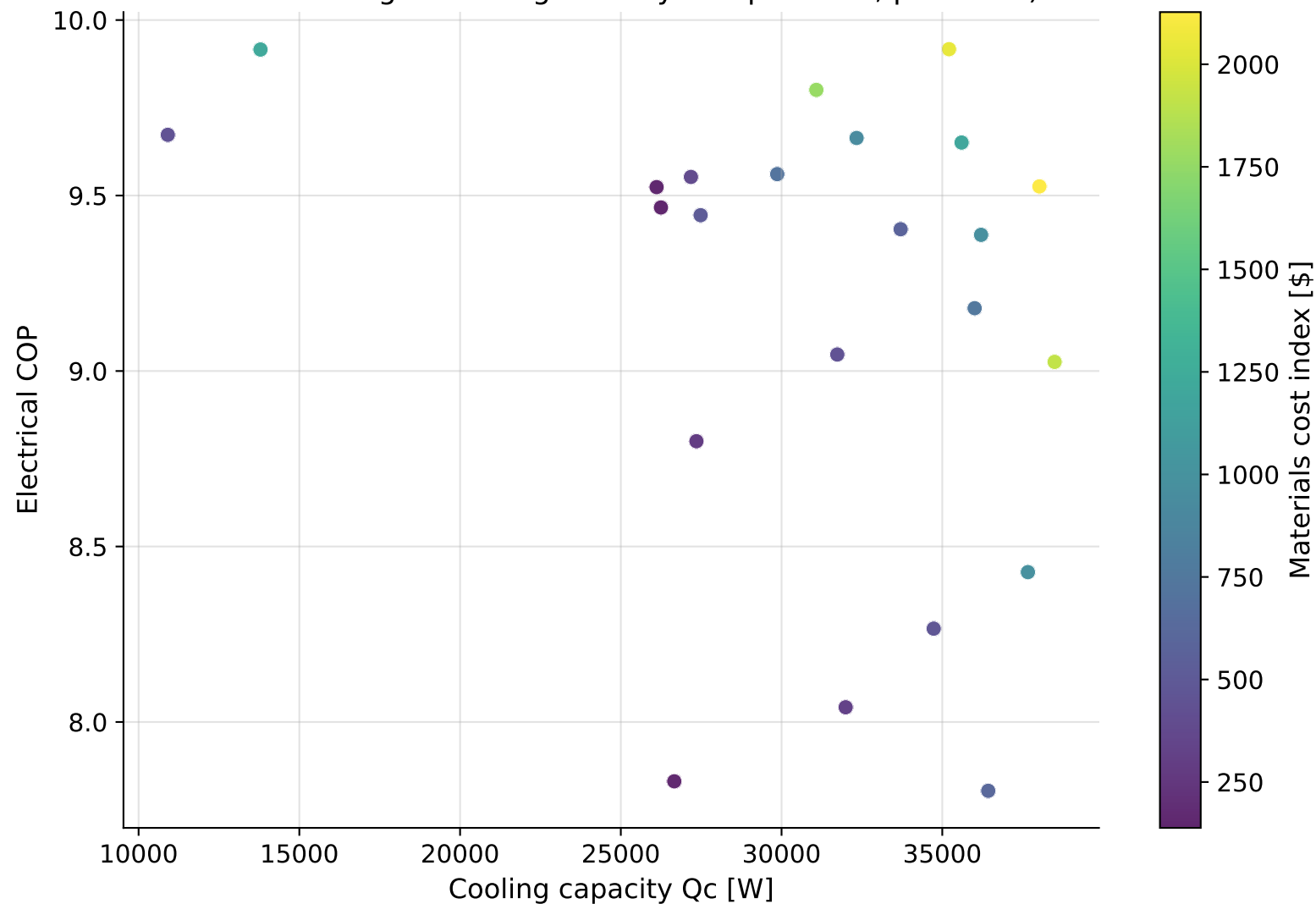
NSGA-III Pareto-Optimal AMR Designs ( T_{\text{cold}}=291\text{K} , span=10K; state-dependent loss + NTU thermal model; material + regenerator geometry co-optimized, phase 15)
