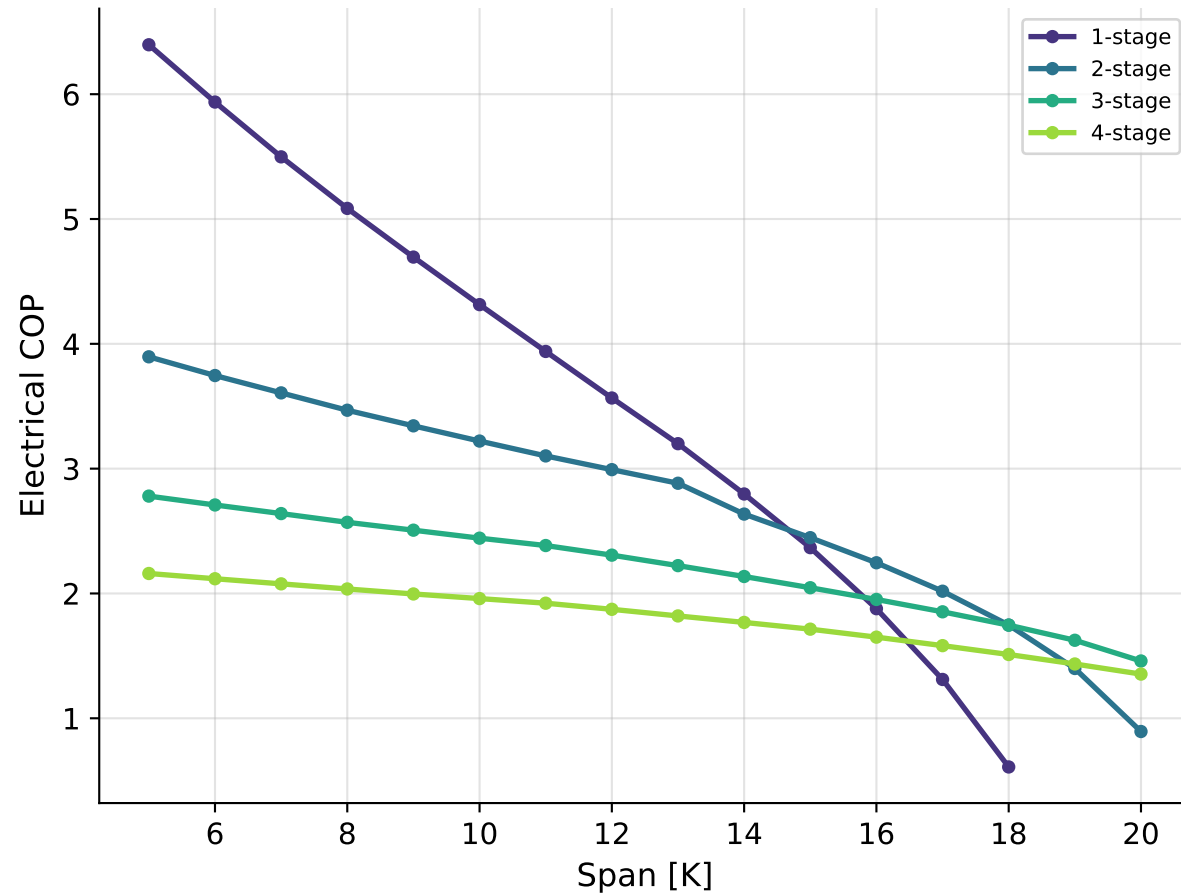
Curie-Graded Cascade COP
