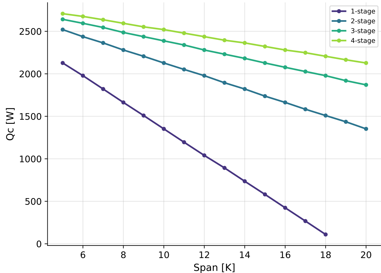
Curie-Graded Cascade Cooling Capacity
