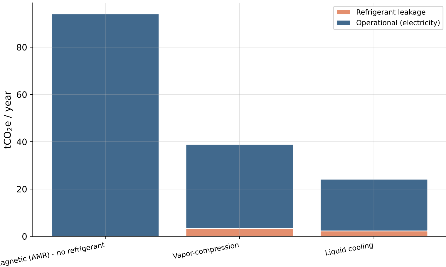
Annual Emissions Comparison, 100kW Cooling Capacity (COPs from the ASHRAE 10K-span operating point)
