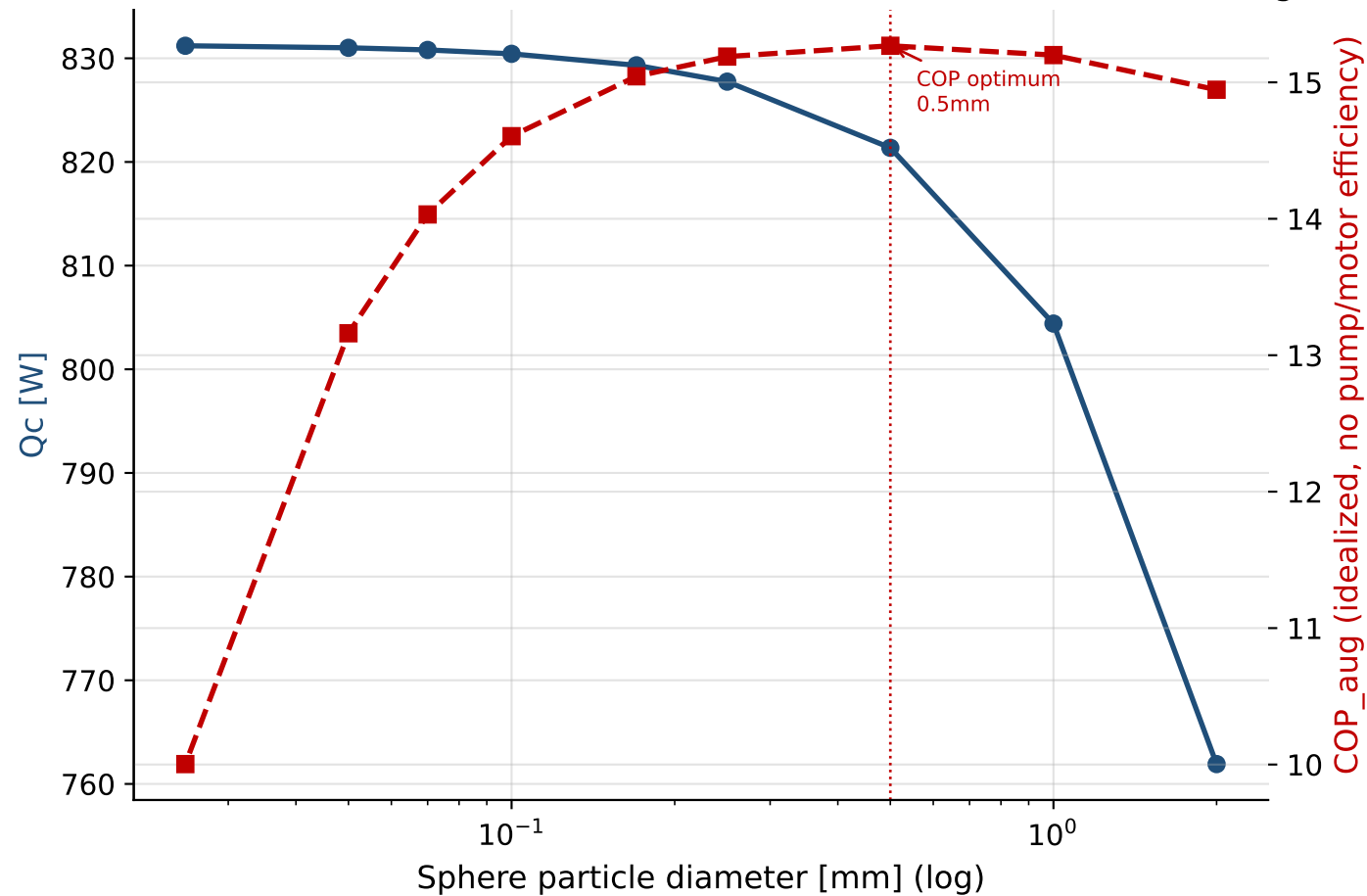
Packed-Bed Geometry Trade-off (Tušek, Kitanovski, Poredoš 2013 friction correlation; fixed \dot{m}=0.08\text{kg/s} )
