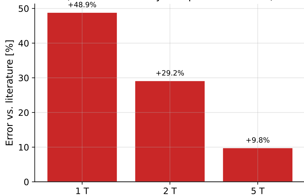
Model Error (mean-field theory overpredicts near T_c )
