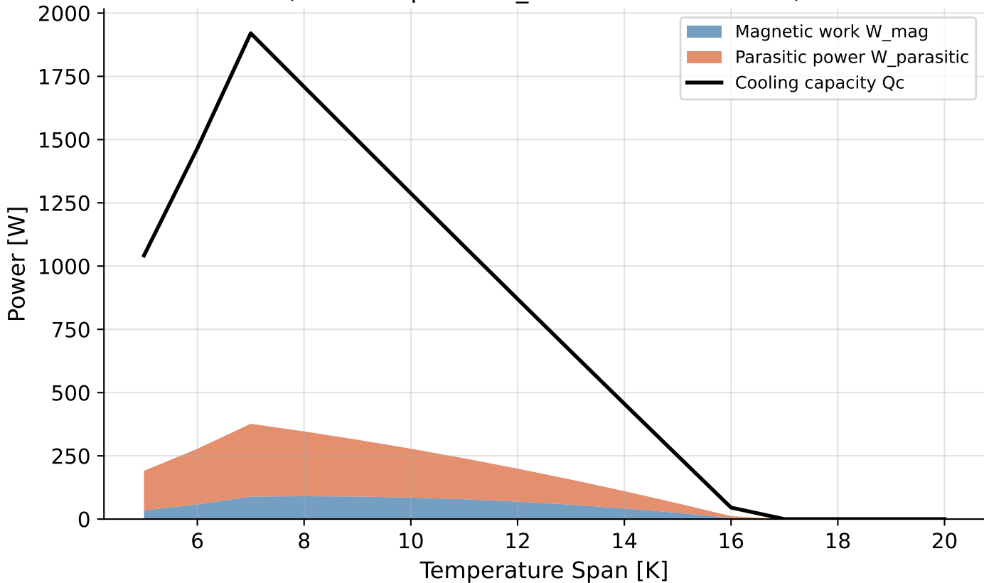
AMR Energy Balance vs. Span (constant parasitic_fraction=0.15 default)
