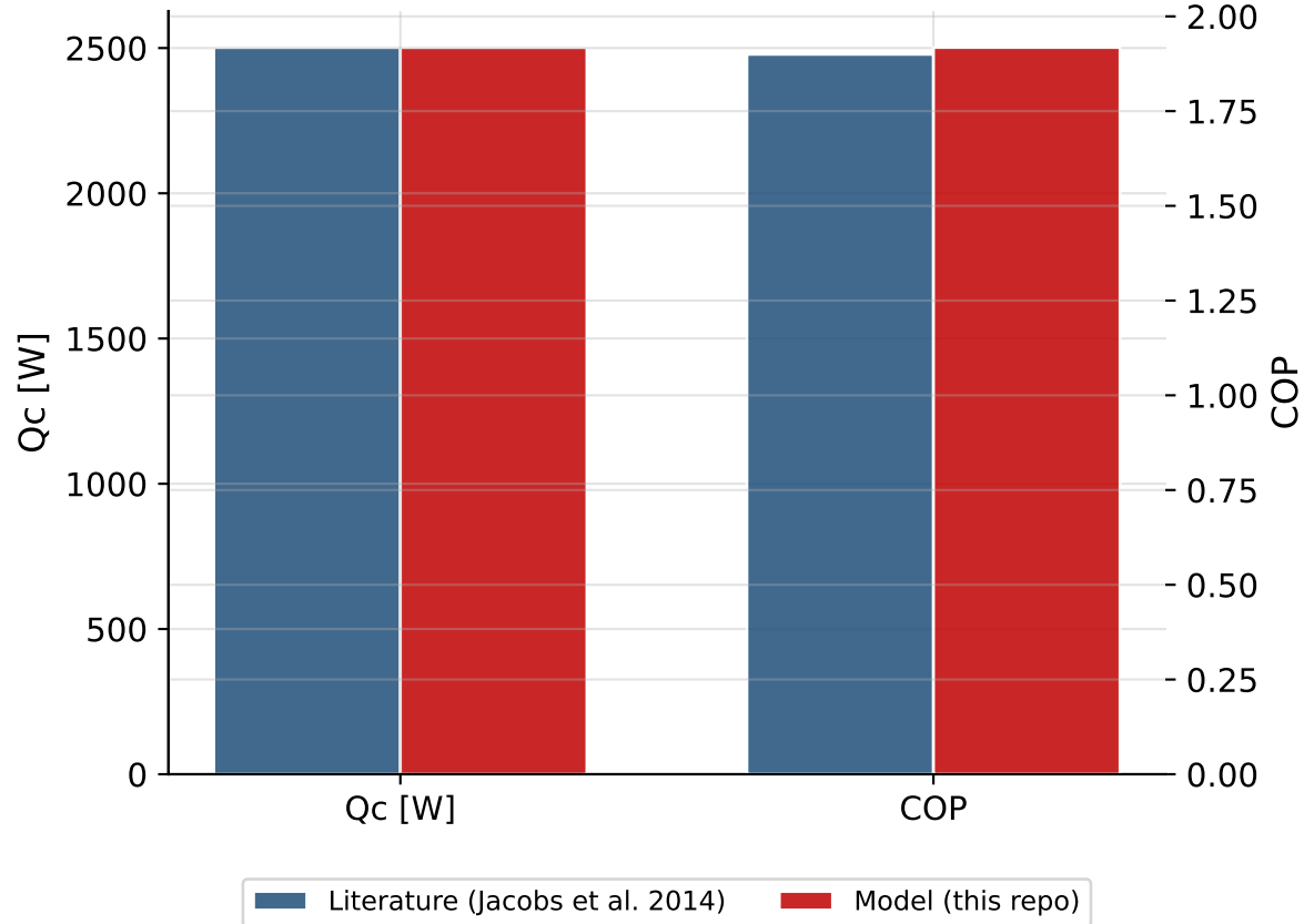
Astronautics_rotary_2014 Validation COP error: +0.9%
