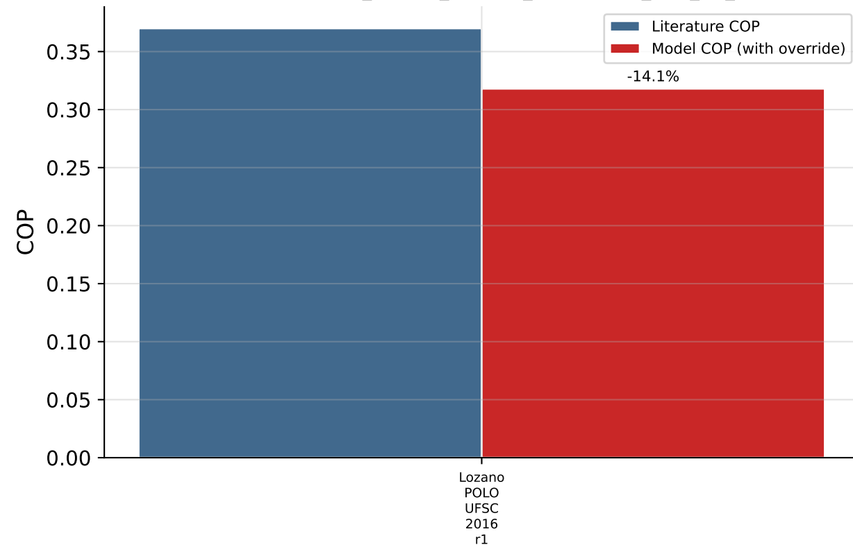
COP Recovered by the Override (% label = model error vs. literature) Still infeasible: DTU_Eriksen_MAGGIE_2016, Risoe_DTU_Gd_2011
