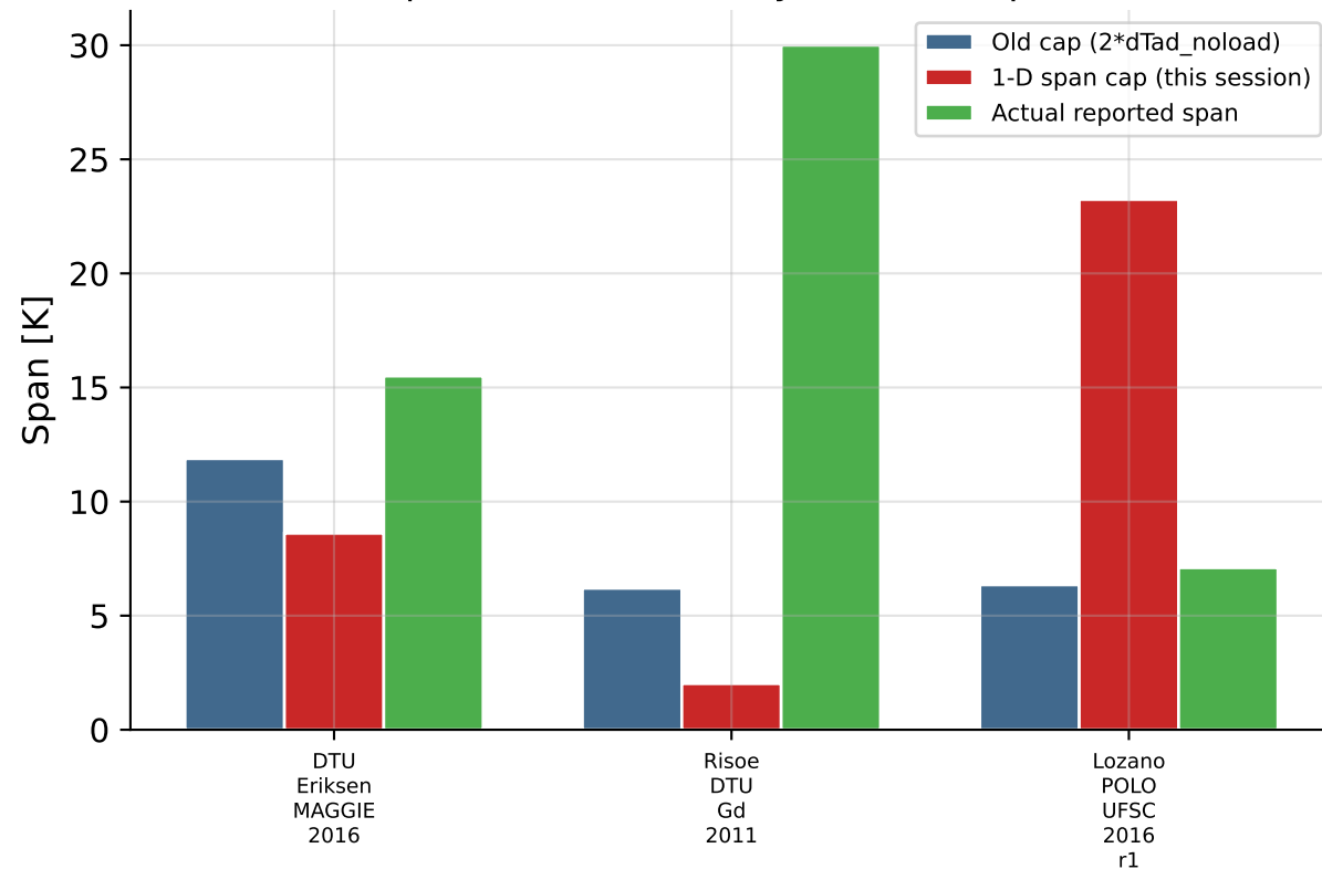
Span Reach: Old Cap vs. 1-D Model vs. Reality (bar at "actual span" not reached by the 1-D cap = still infeasible)
