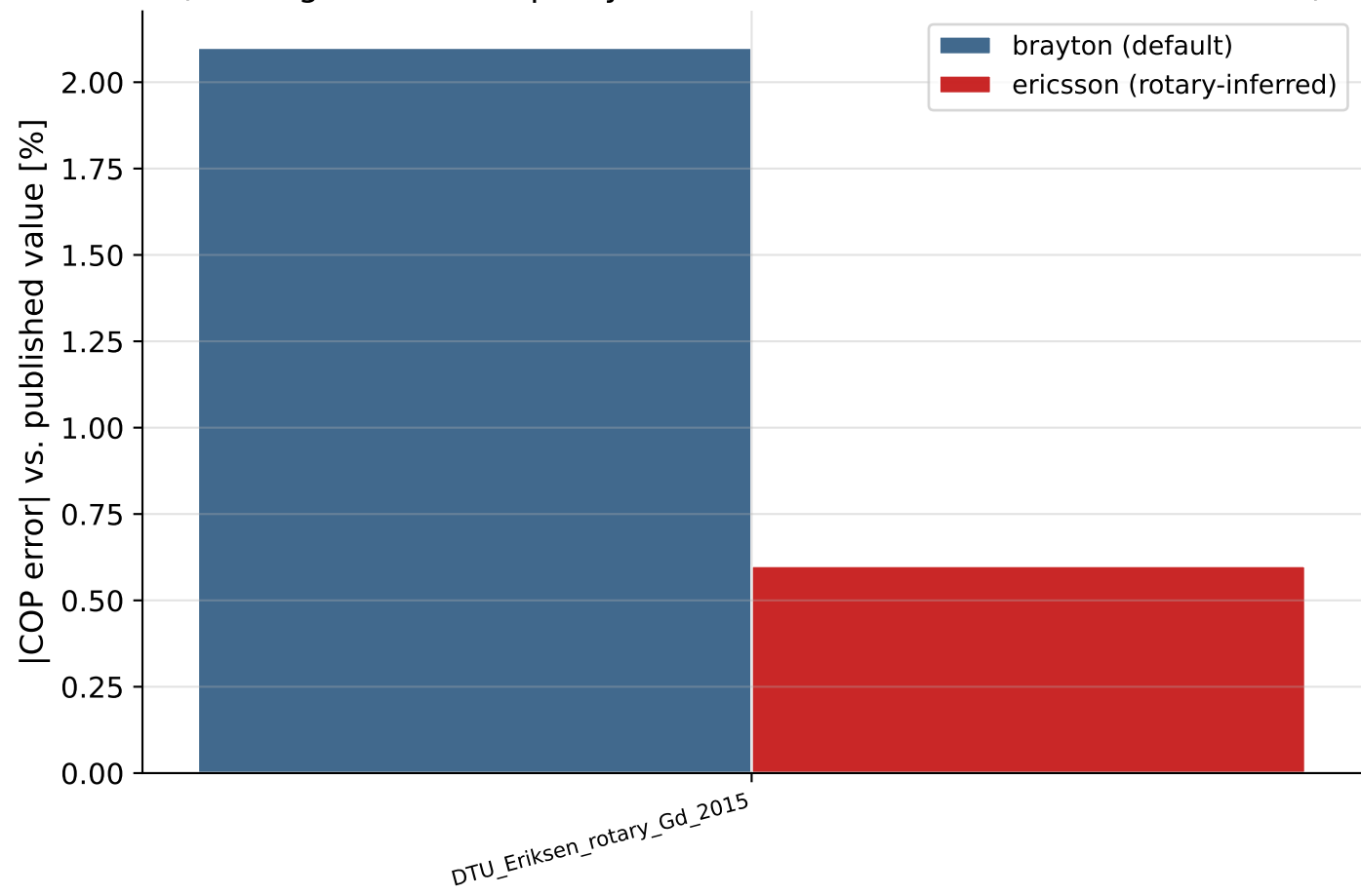
Cycle-Topology Sensitivity: Rotary Benchmark Devices (naming-convention proxy, not a literature-confirmed classification)
