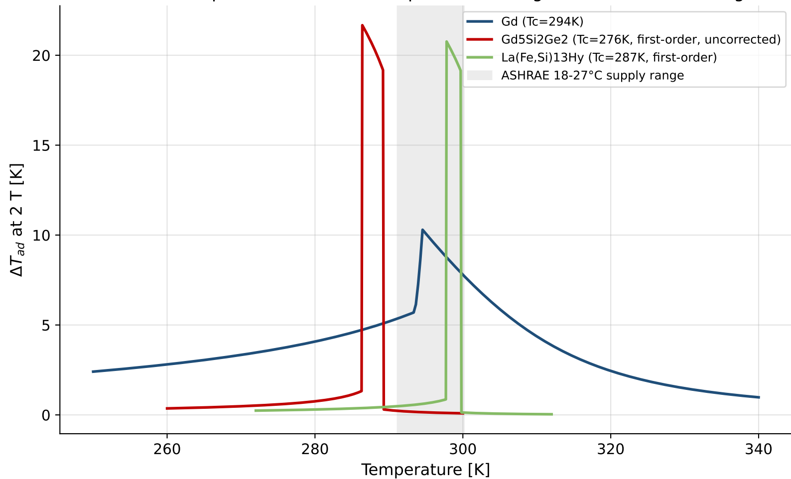
Material Comparison: Adiabatic Temperature Change vs. Data-Center Range
