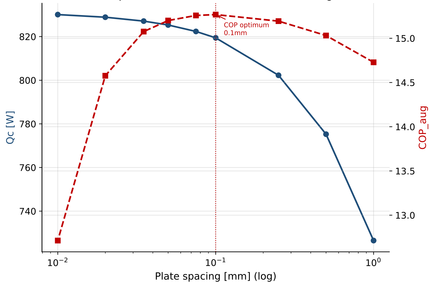
Parallel-Plate Geometry Trade-off (fixed plate thickness=0.25mm, \dot{m}=0.08\text{kg/s} )
