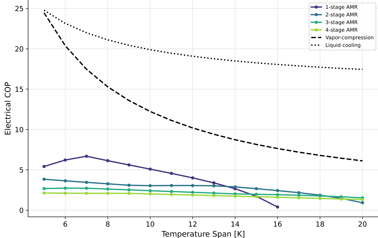
Multi-Stage Cascade AMR vs. Baselines (Gd, 2T, 5kg/stage)
