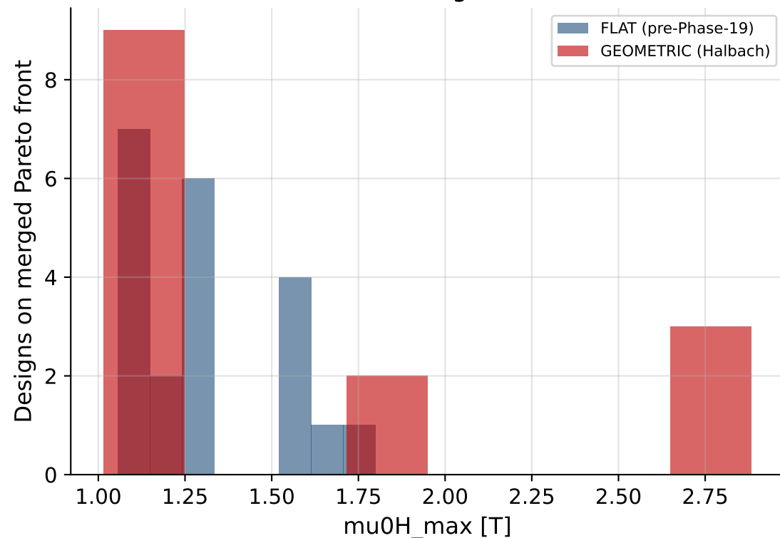
Field-Strength Distribution FLAT vs. GEOMETRIC magnet-mass cost term
