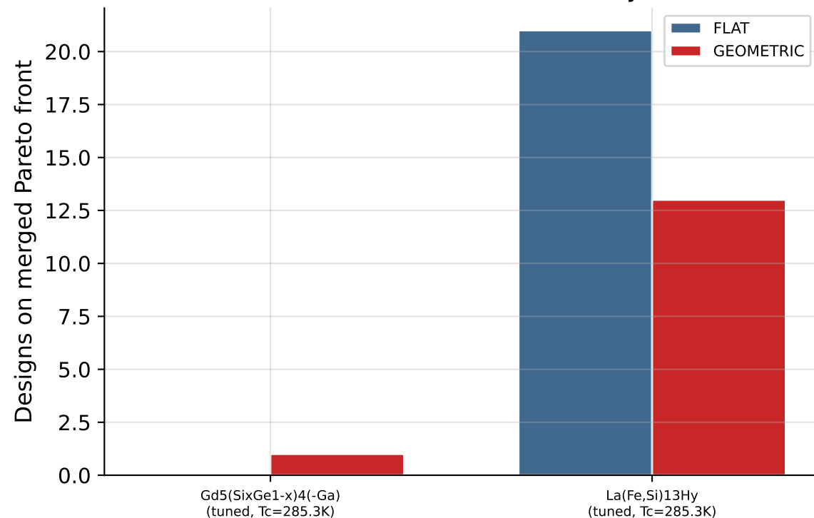
Material-Selection Sensitivity
